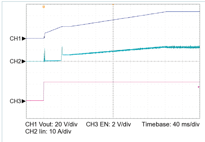
Figure 15 — Startup from EN, V_{IN} = 28\text{ V} , C_{OUT\_EXT} = 2000\text{ }\mu\text{F} , R_{LOAD} = 7.200\text{ }\Omega
