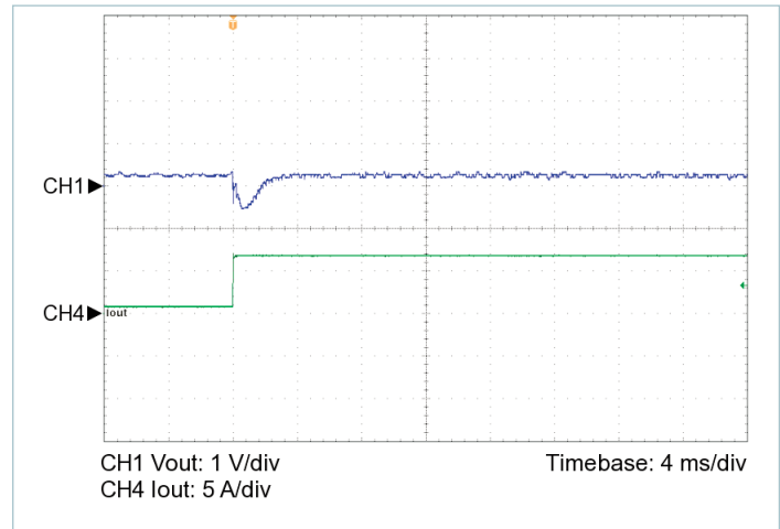
Figure 6 — 10% to 100% load transient response, V_{IN} = 28\text{ V} , nominal trim, C_{OUT\_EXT} = 200\text{ }\mu\text{F}
