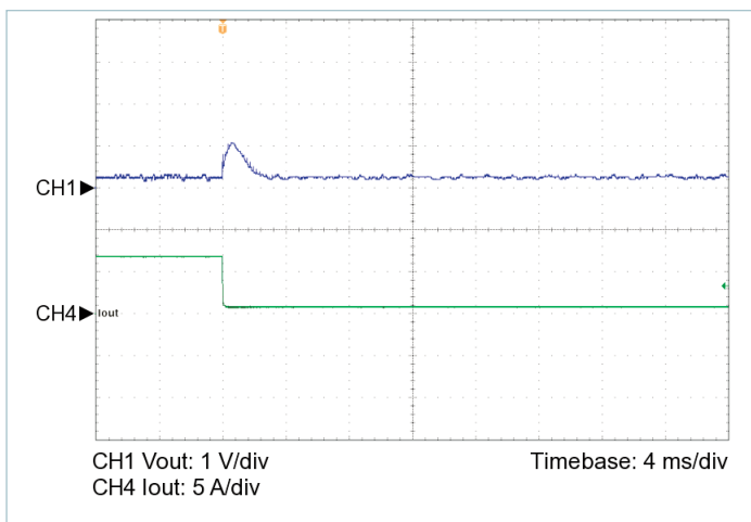
Figure 5 — 100% to 10% load transient response, V_{IN} = 28\text{ V} , nominal trim, C_{OUT\_EXT} = 200\text{ }\mu\text{F}
