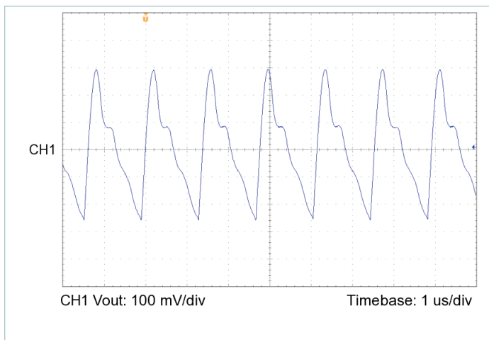
Figure 17 — Output voltage ripple, V_{IN} = 28\text{ V} , V_{OUT} = 48.0\text{ V} , C_{OUT\_EXT} = 200\text{ }\mu\text{F} , R_{LOAD} = 7.200\text{ }\Omega
