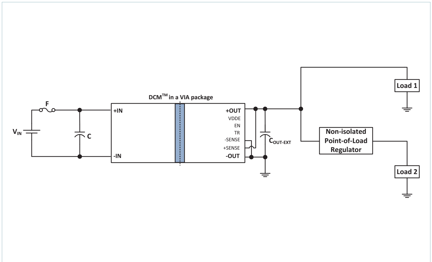
Typical Application: Single DCM3414x50M53C2yzz in Local Sense Operation, to a non-isolated regulator, and direct to load
