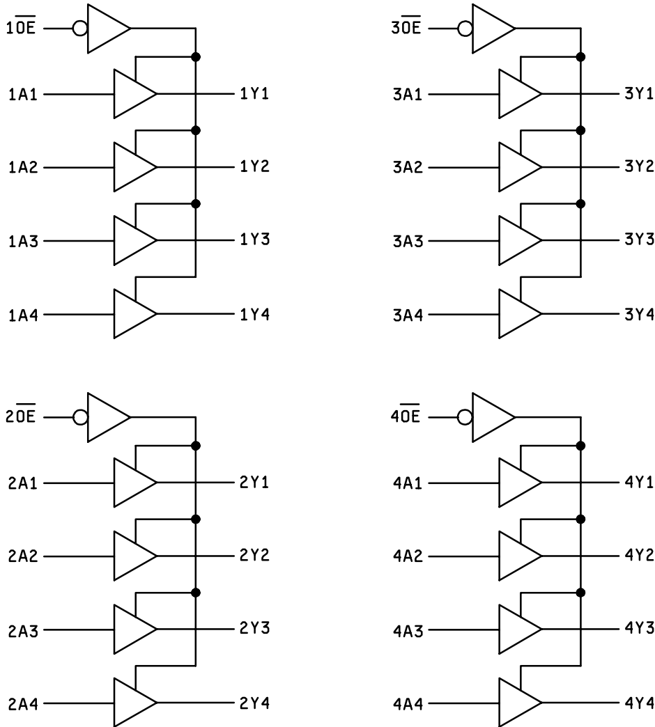
FIGURE 3. Logic diagram.
