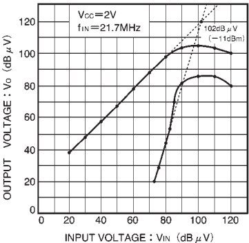
Fig. 5 Mixer output voltage vs. input voltage
