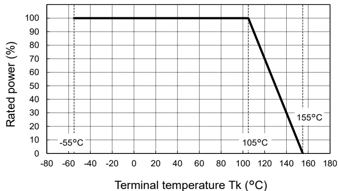
Fig.3< Terminal temperature>
