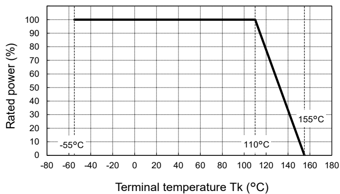
Fig.3< Terminal temperature>
