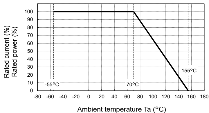
Fig.2< Terminal temperature>
