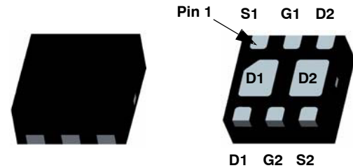
WDFN6 2x2, 0.65P (MicroFET™ 2x2) CASE 511DA
