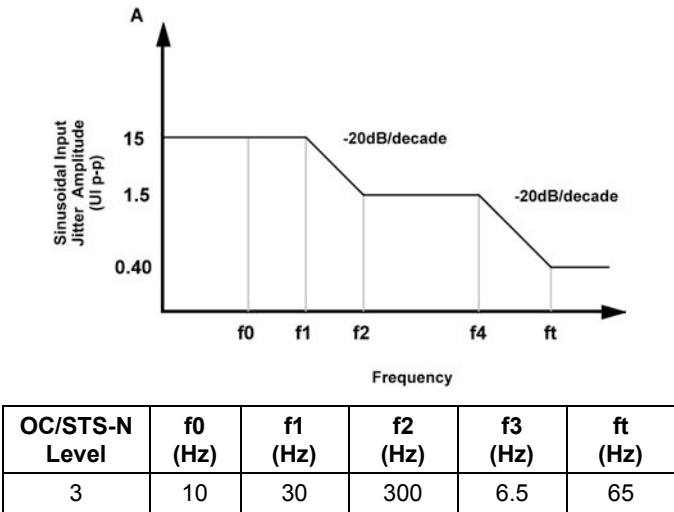
Figure 1. Input Jitter Tolerance
