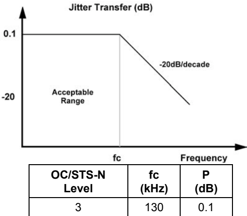
Figure 2. Jitter Transfer
