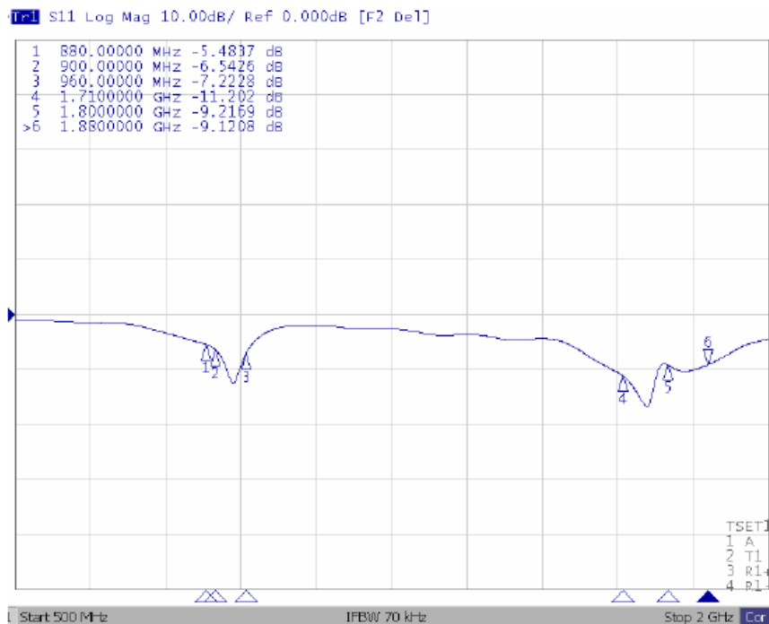
Fig. 4 Return loss
