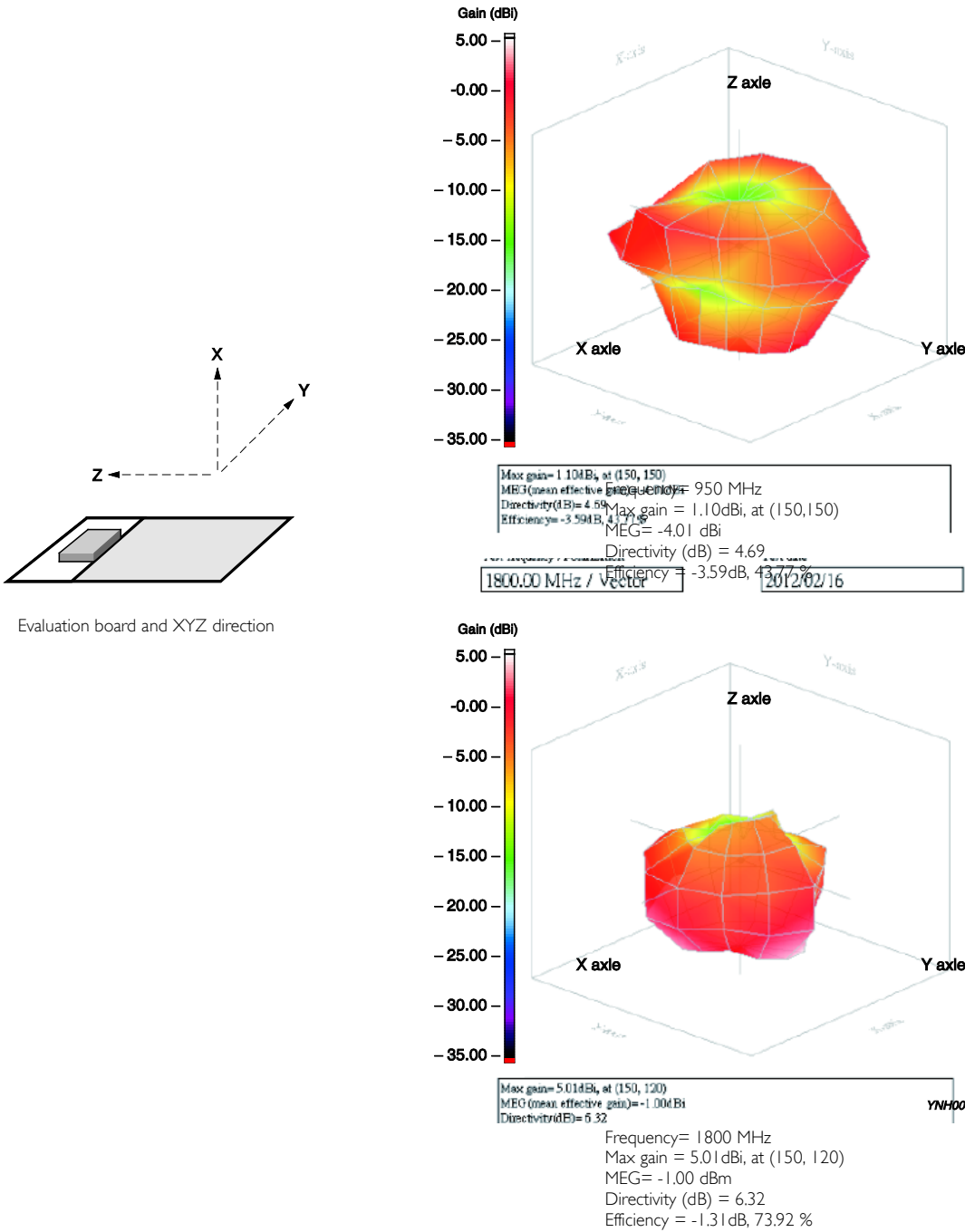
Fig. 5 Radiation pattern
