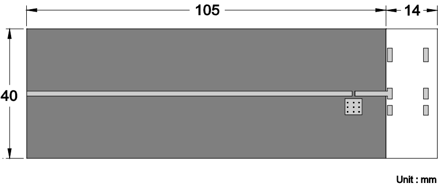
Fig. 2 Outlook and dimension of evaluation board
