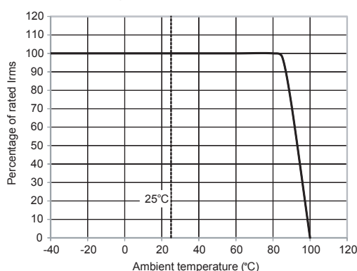
Irms derating
