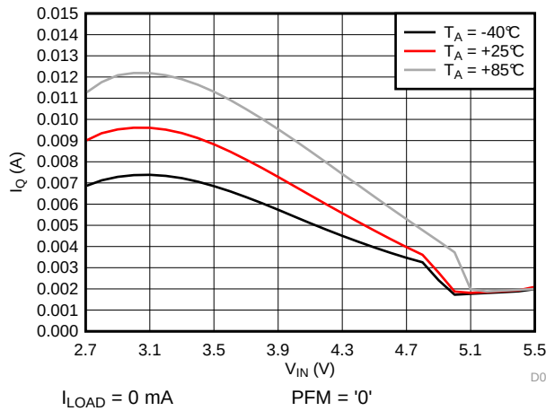
Figure 9. PWM Quiescent Current
