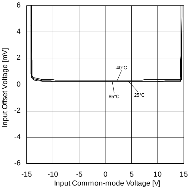
Figure 9. Input Offset Voltage vs Input Common-mode Voltage (VCC/VEE=±15V)
