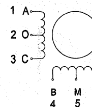
Wiring Diagram
