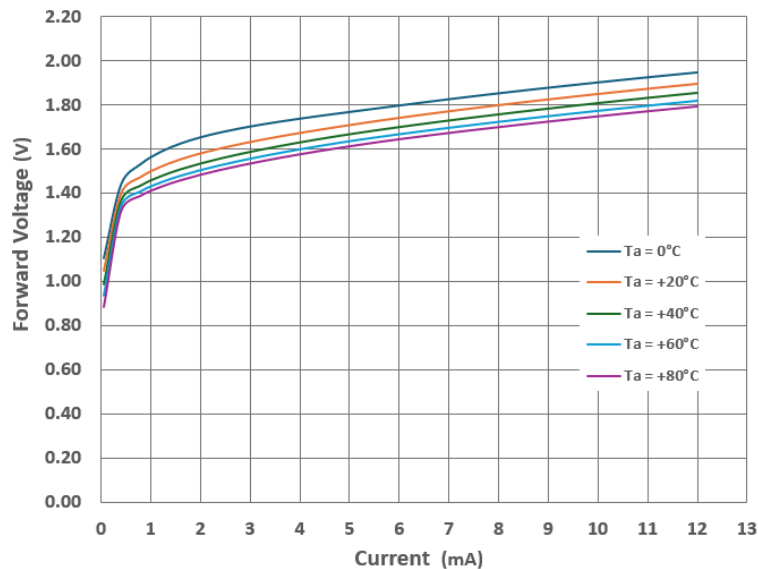
OPB608V VCSEL Forward Voltage vs Current
