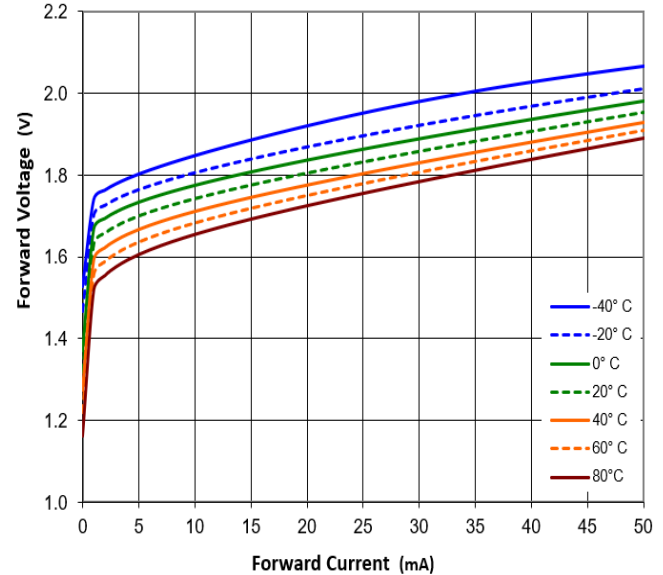
OPB608R Forward Voltage vs Current vs Temperature
