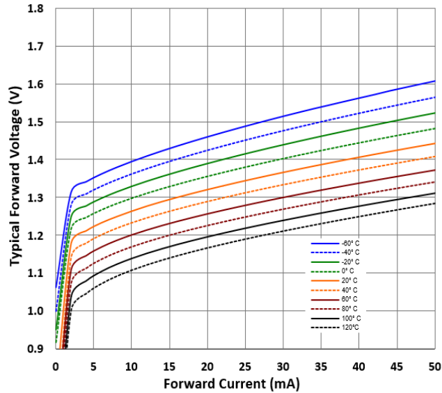
OPB608 LED Forward Voltage vs I_f vs Temp
