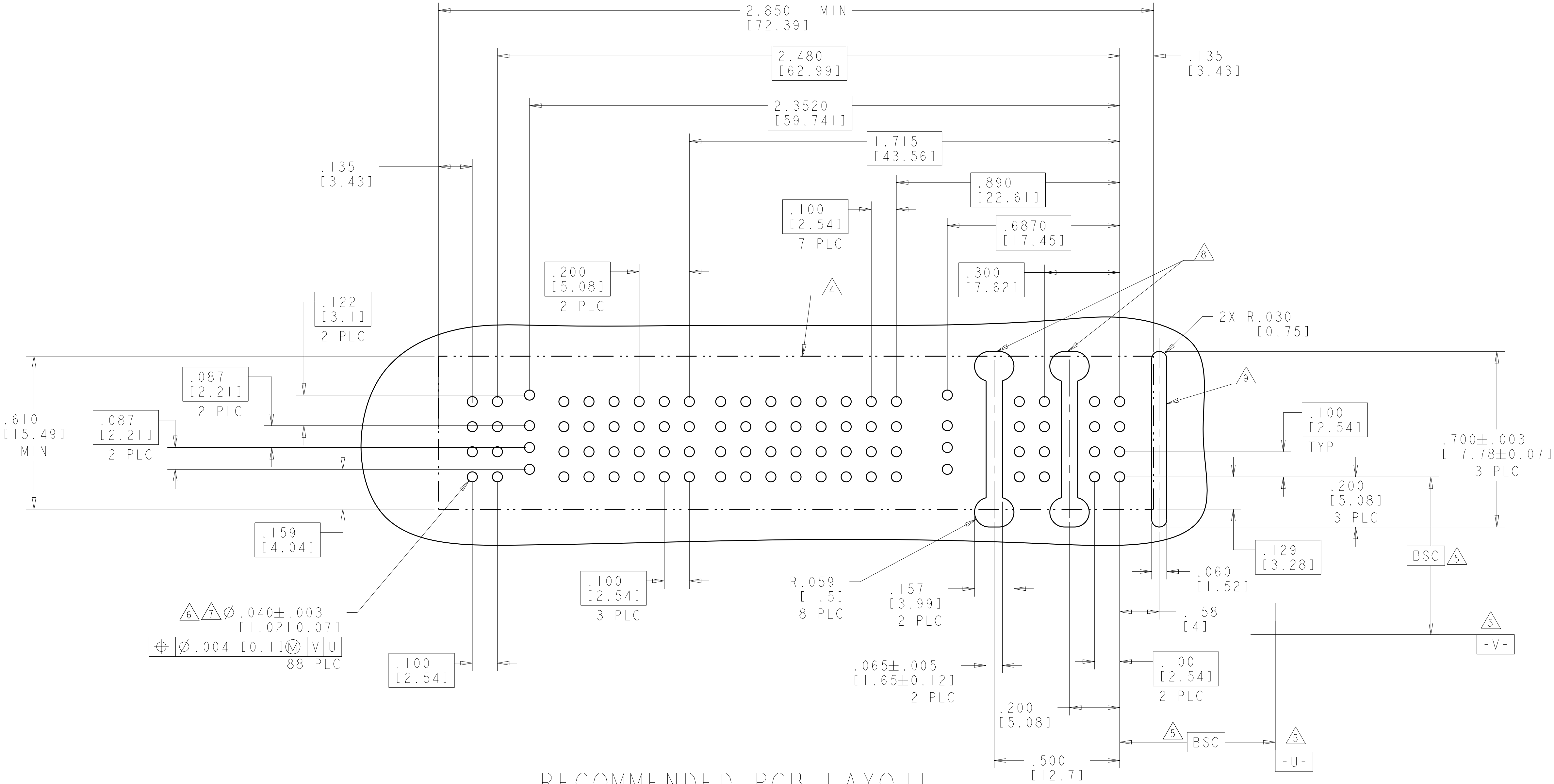
RECOMMENDED PCB LAYOUT
