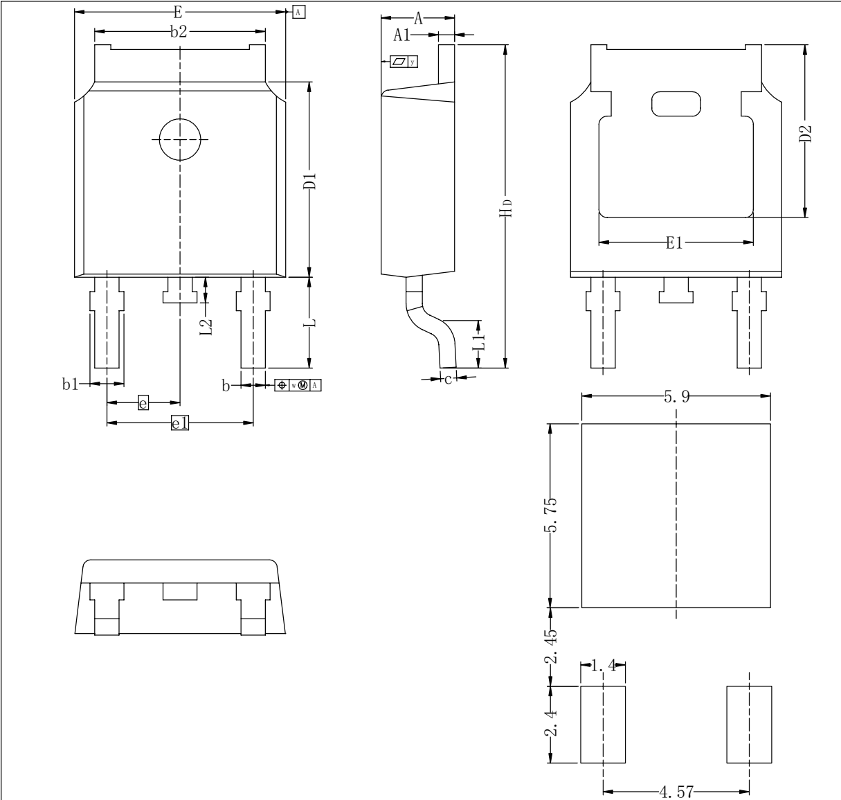
Plastic single-ended surface-mounted package (DPAK); 3 leads (one lead cropped)
