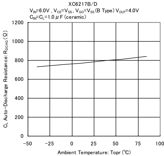
(7) CL Auto-Discharge Resistance vs. Ambient
