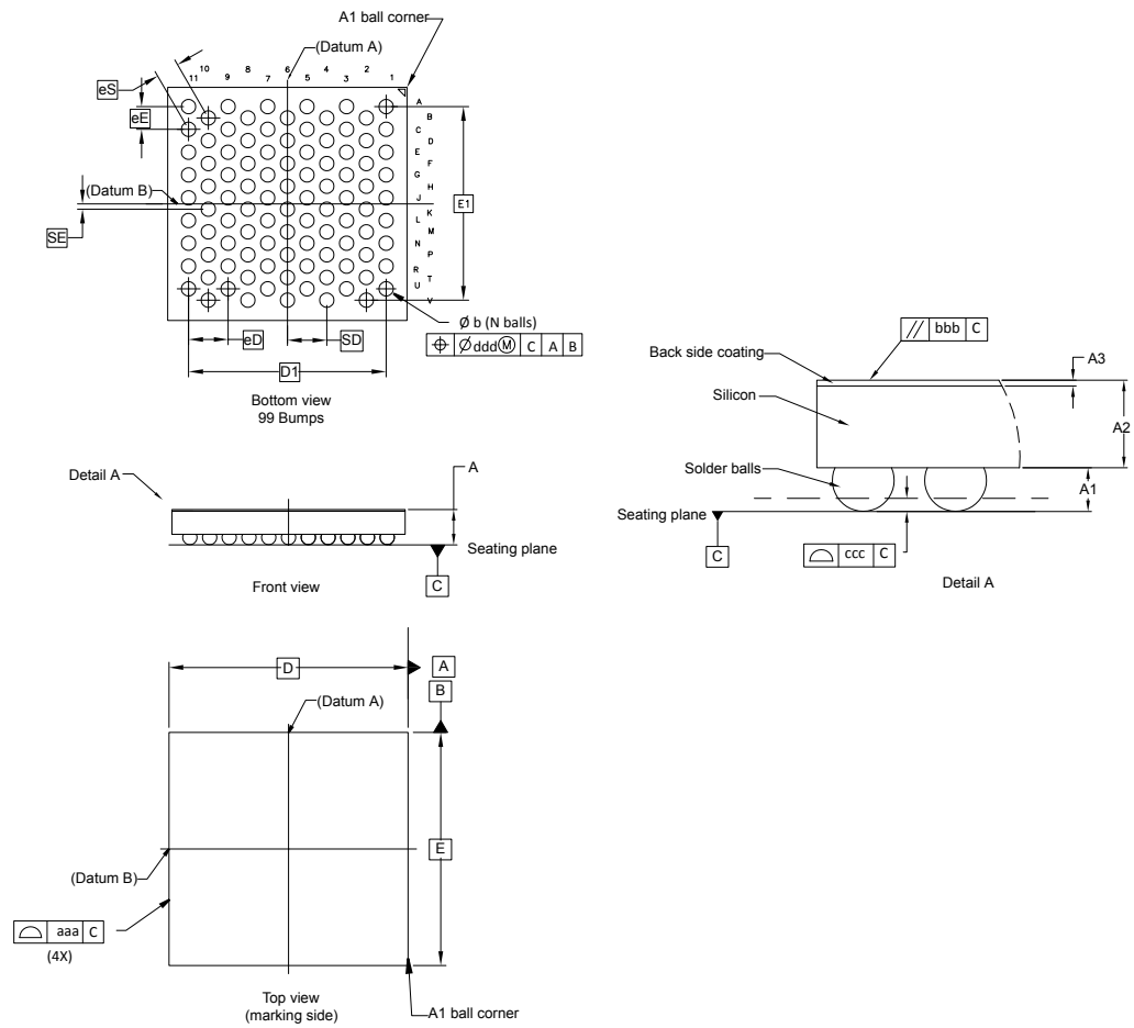
Figure 73. WLCSP99 - Outline
