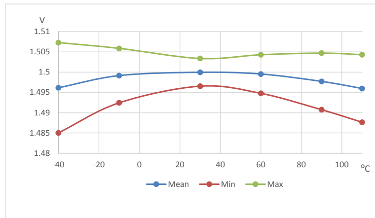
Figure 41. VREFBUF_OUT versus temperature (VRS = 000)
