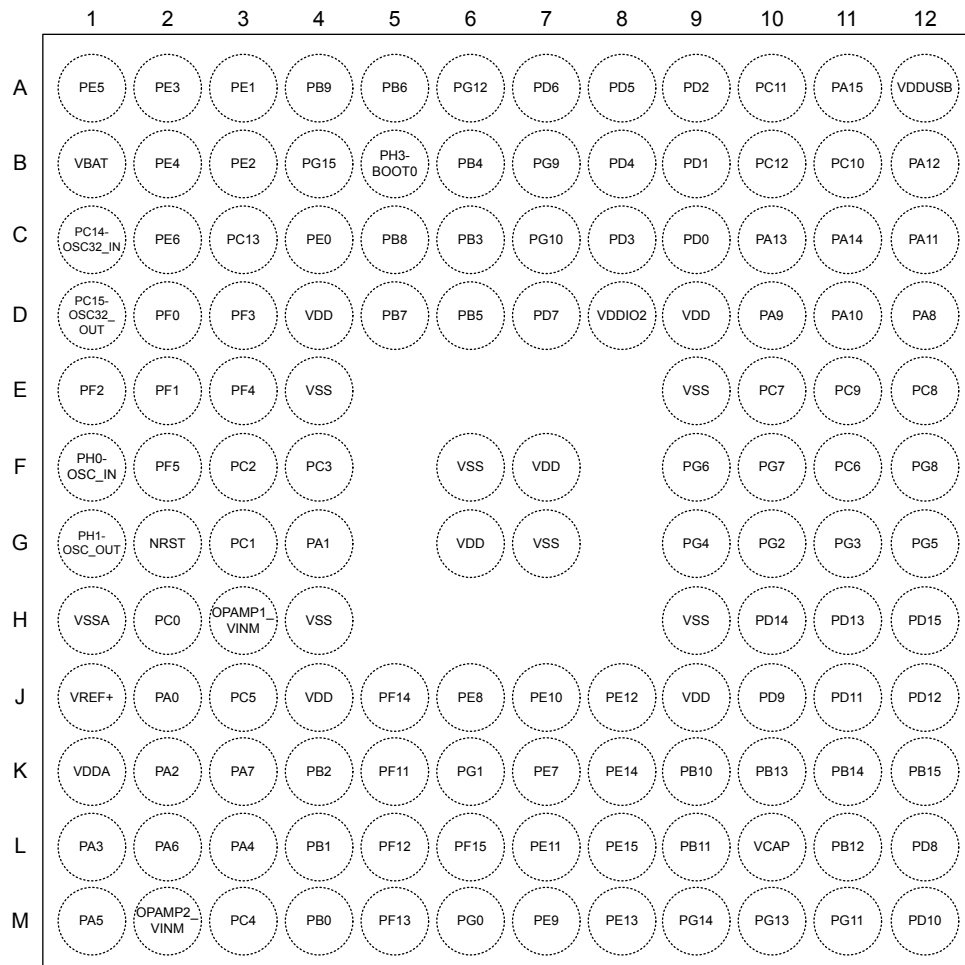
Figure 18. UFBGA132 ballout
