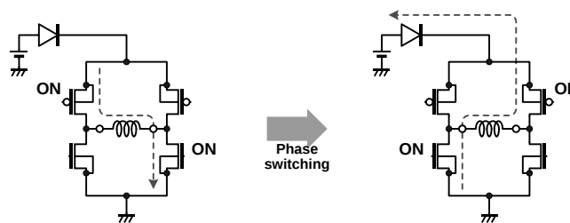
Figure 28. VCC voltage rise by back electromotive force
