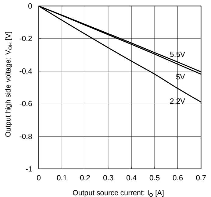
Figure 12. Output high side voltage ( Temp=25^{\circ}C )
