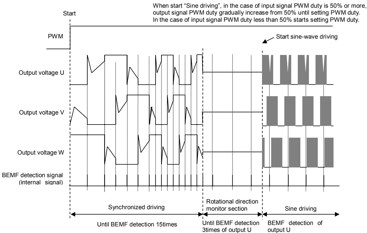
Figure 18. Timing chart at startup
