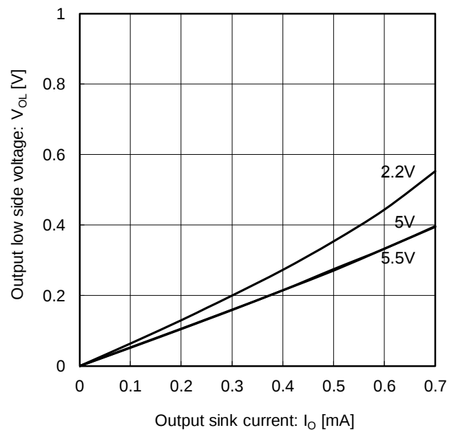
Figure 14. Output low side voltage ( Temp=25^{\circ}C )
