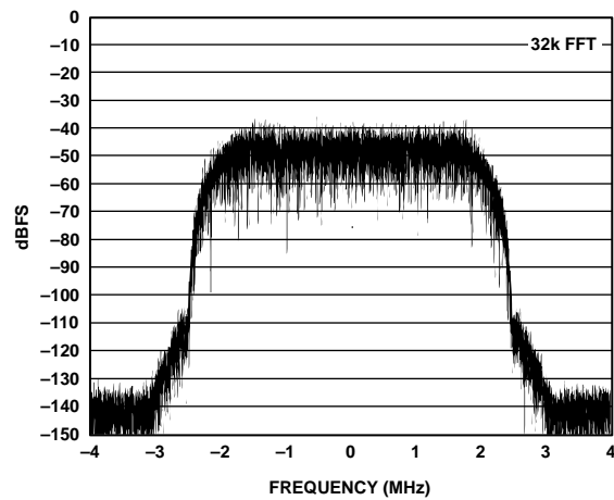
Figure 7. WCDMA Carrier A_{IN} = 169\text{ MHz} ; Encode = 61.44 MSPS
