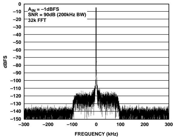
Figure 2. GSM/EDGE with Single Tone A_{IN} = 30\text{ MHz} ; Encode = 61.44 MSPS
