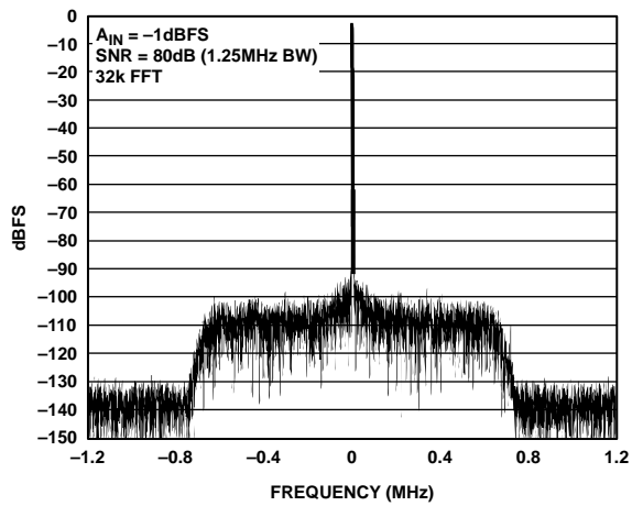
Figure 3. CDMA2000 with Single Tone A_{IN} = 76\text{ MHz} ; Encode = 61.44 MSPS
