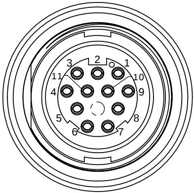
FACE VIEW W4281-11SG-3ES 11-POS.
