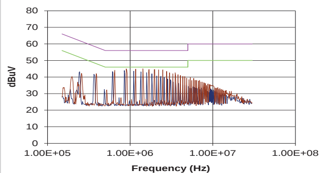
CRE1S0505MC
