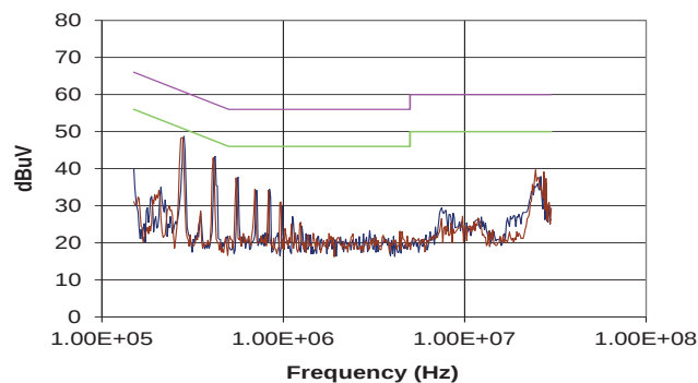
CRE1S0505MEC
