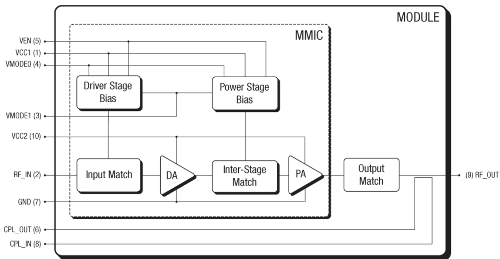
Figure 1. SKY77761-11 Functional Block Diagram
