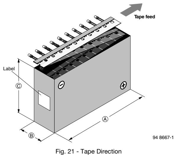
Fig. 21 - Tape Direction
