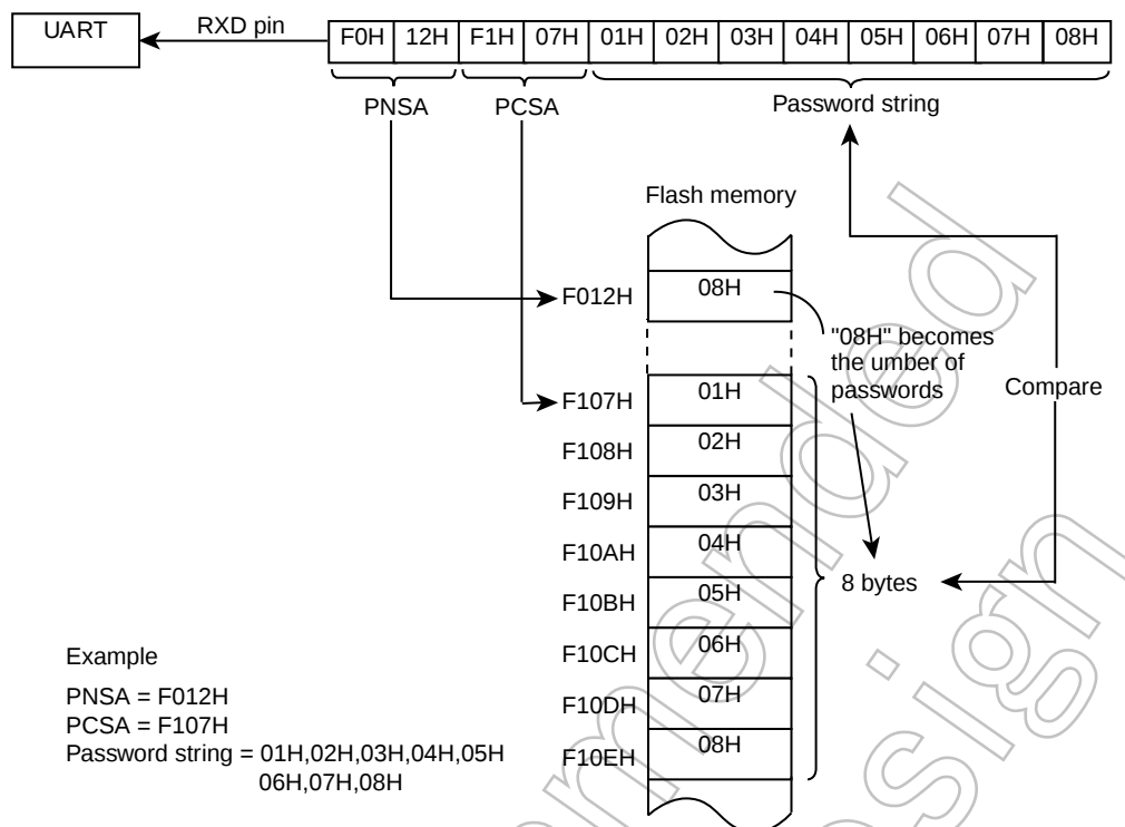
Figure 15-5 Password Comparison
