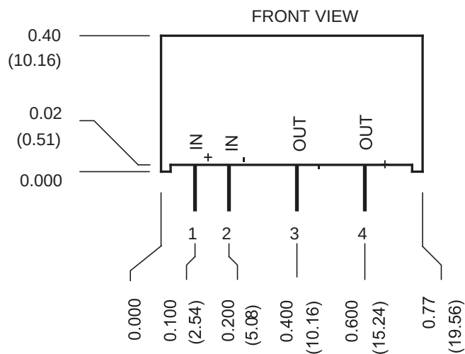
Figure 3. Mechanical Dimensions
