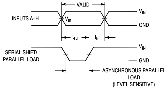
Figure 7. Parallel-Load Mode
