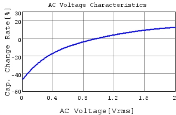
GRT155R61E474KE01 C-AC Voltage capchange, D
