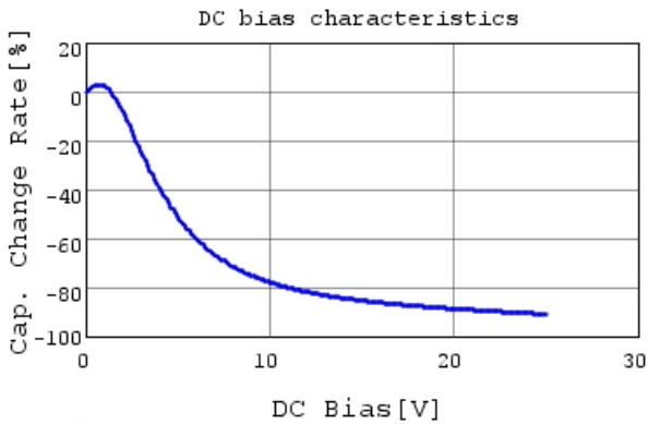
GRT155R61E474KE01 C-DC bias capchange, 25.0c
