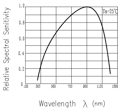
Fig.5 Spectral Sensitivity
