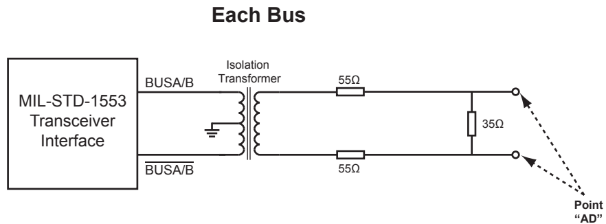
Figure 24. MIL-STD-1553 Direct Coupled Test Circuits
