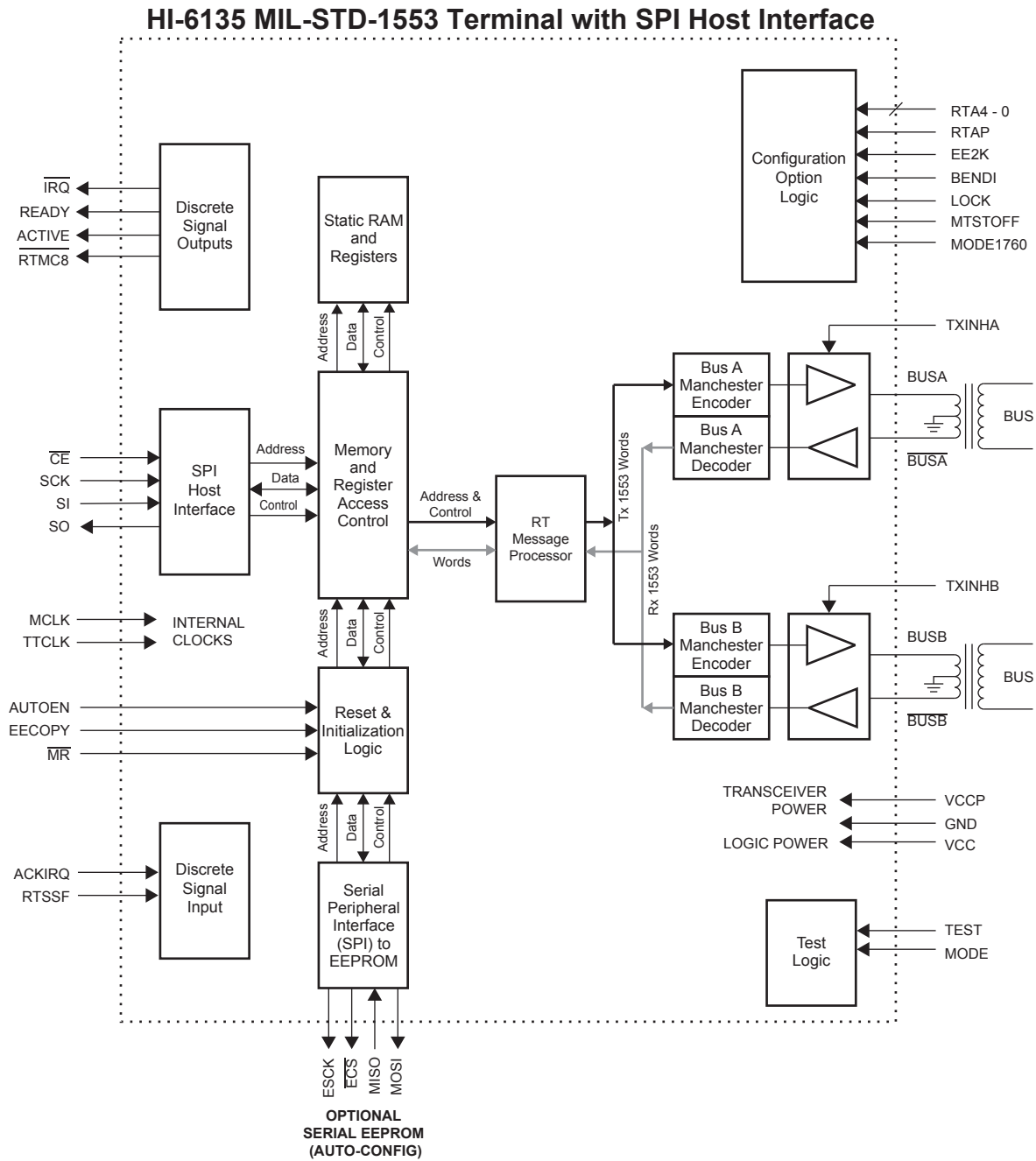
Figure 1. Block Diagram
