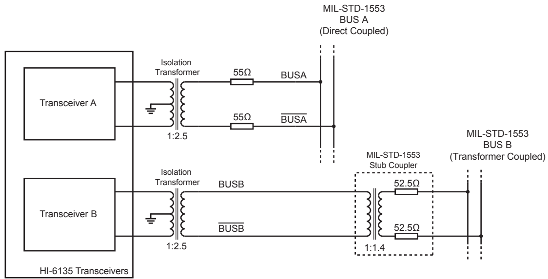
Figure 23. Bus Connection Example using HI-6135
