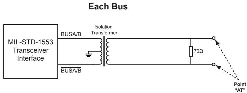
Figure 25. MIL-STD-1553 Transformer Coupled Test Circuits
