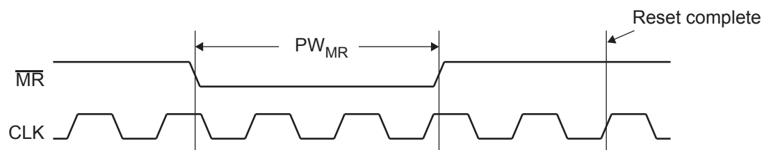
Figure 22. MR Master Reset Timing Diagram
