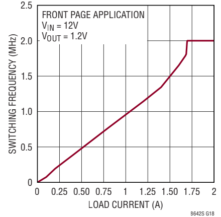
Burst Frequency
