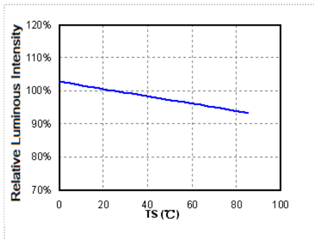
5. Relative Luminous Intensity vs. Solder Temperature ( I_F=20\text{mA} )
