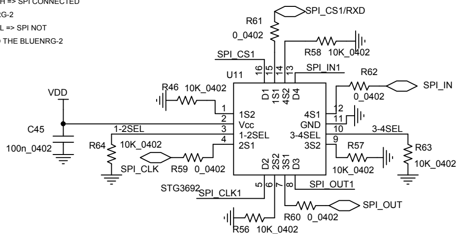
Figure 11. STEVAL-IDB008V2 - Switch
