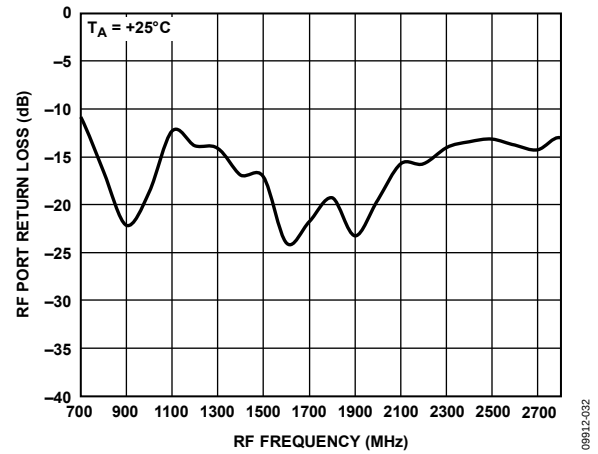
Figure 32. RF Port Return Loss, Fixed IF vs. RF Frequency
