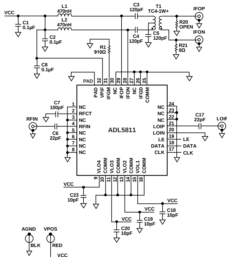
Figure 59. Basic Connections
