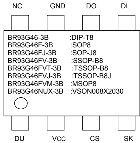
Figure 3. Pin Configuration
