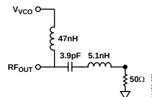
Figure 22. Optimum ADF4360-5 Output Stage
