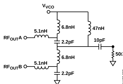
Figure 23. Balun for Combining ADF4360-5 RF Outputs
