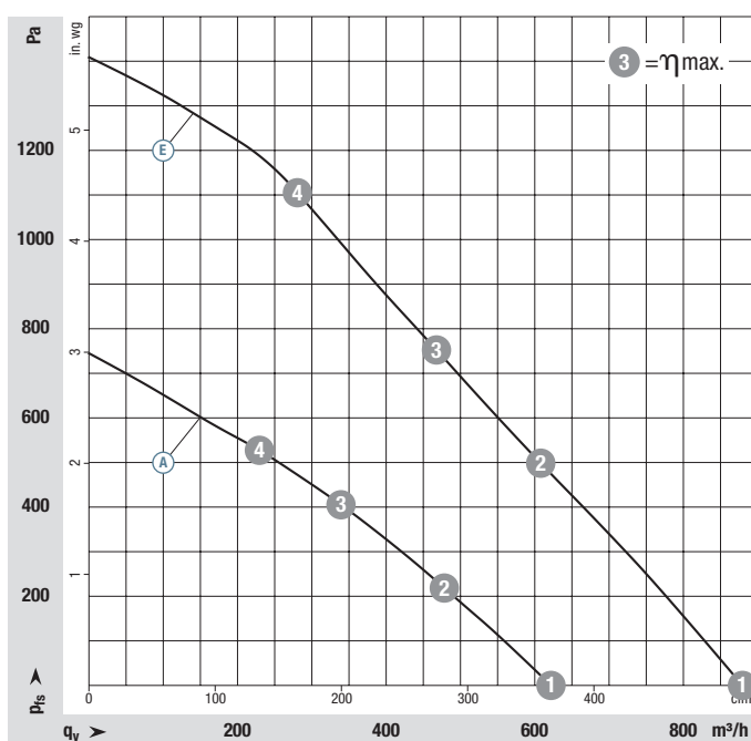
Curves: Sensor-controlled MODBUS-RTU
