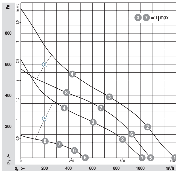
Curves: 2 Speed stages
