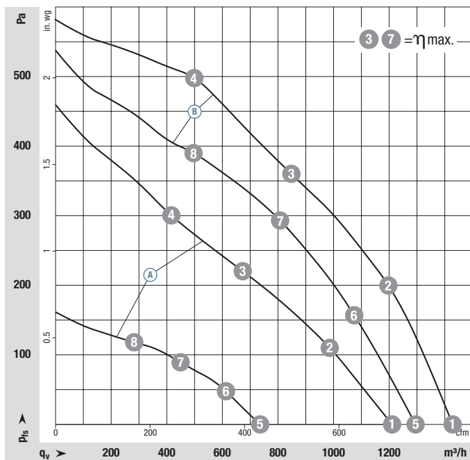
Curves: 2 Speed stages
