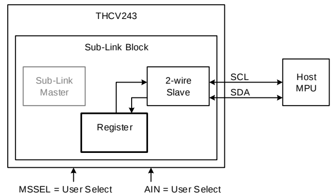
Figure 13. Host to THCV243 local register access configuration
