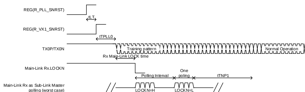
Figure 22. Lock Sequence
