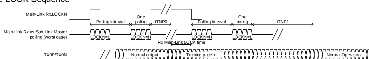
Figure 23. Re-Lock Sequence
