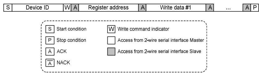
Figure 14. 2-wire serial I/F write to THCV243 local register protocol
