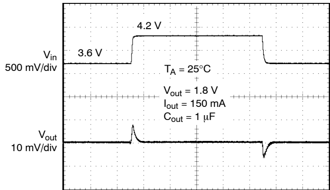
Figure 21. Line Transient
