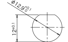
Panel Mounting Dimension
