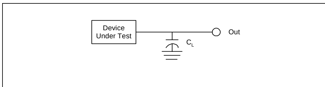
Figure 5. Test Configuration
