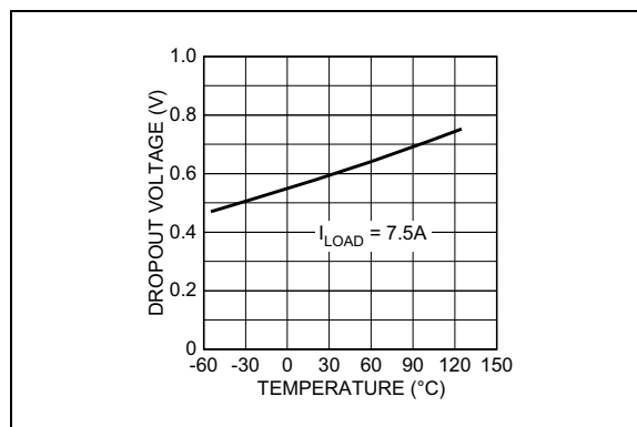
FIGURE 2-6: Dropout Voltage vs. Temperature.
