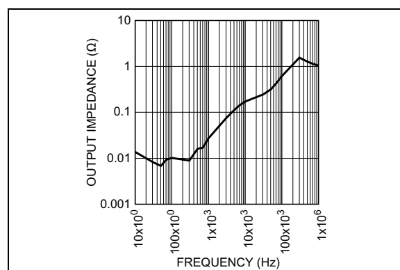
FIGURE 2-16: Output Impedance vs. Frequency.
