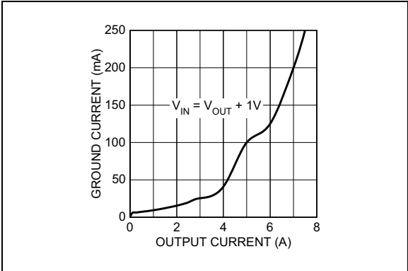
FIGURE 2-12: Ground Current vs. Output Current.
