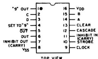
TERMINAL ASSIGNMENT
