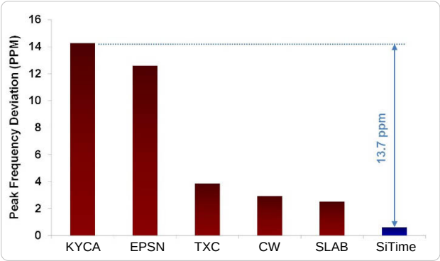
Figure 20. Shock Robustness [6]
