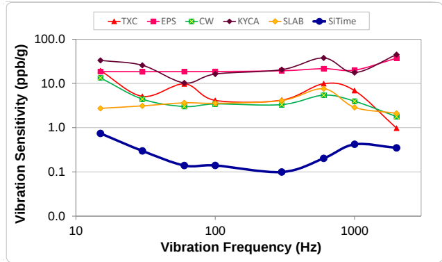
Figure 19. Vibration Robustness [5]
