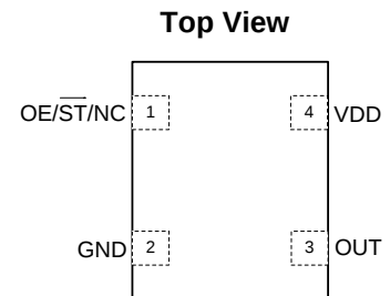
Figure 1. Pin Assignments
