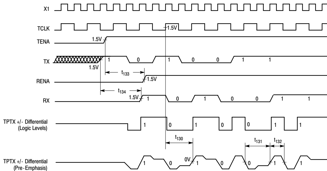
Figure 17. TPTX Transmit Timing (Start of Frame) Switching
