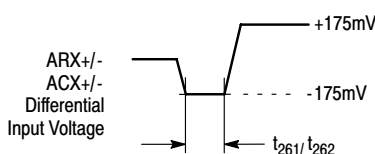
Figure 32. ARX/ACX Timing
