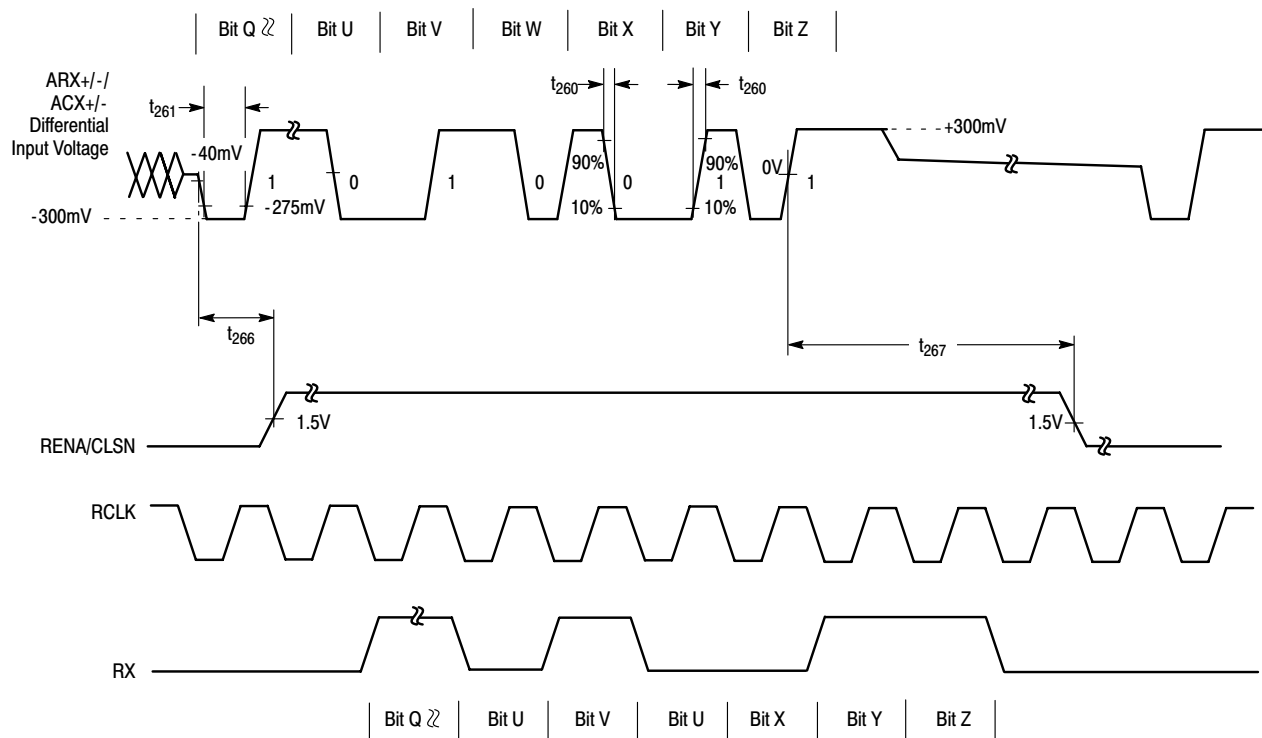
Figure 33. ARX/ACX Timing
