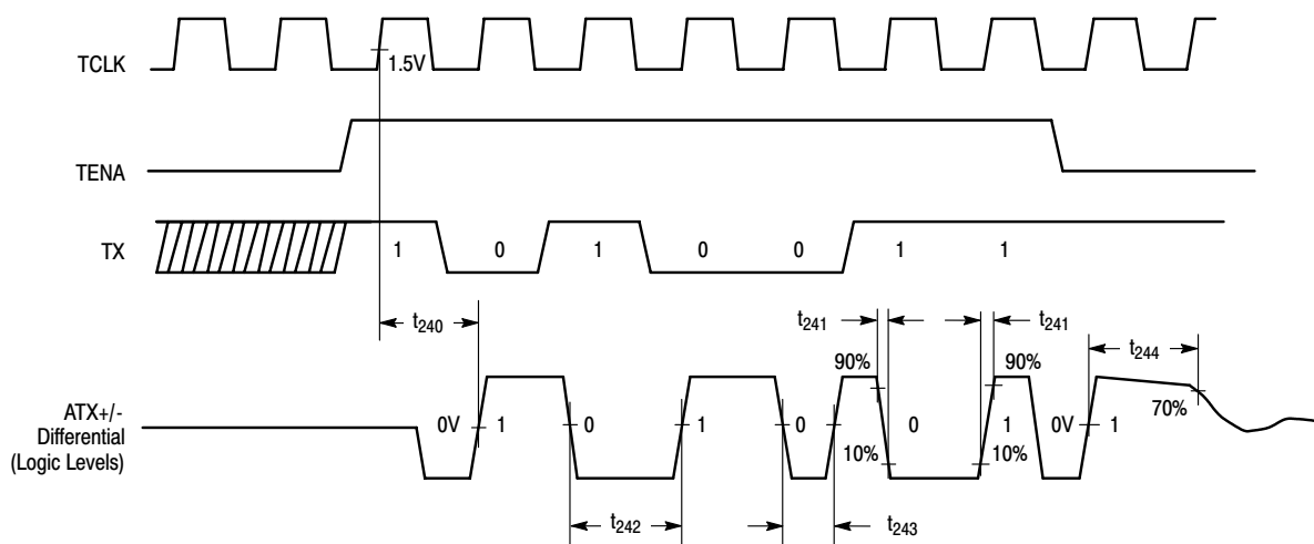
Figure 31. ATX Transmit Timings
