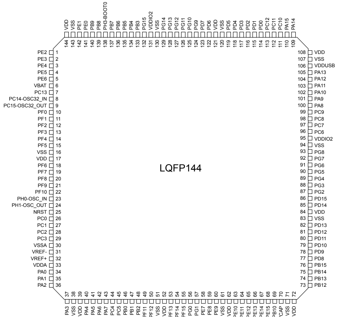
Figure 20. LQFP144 pinout
