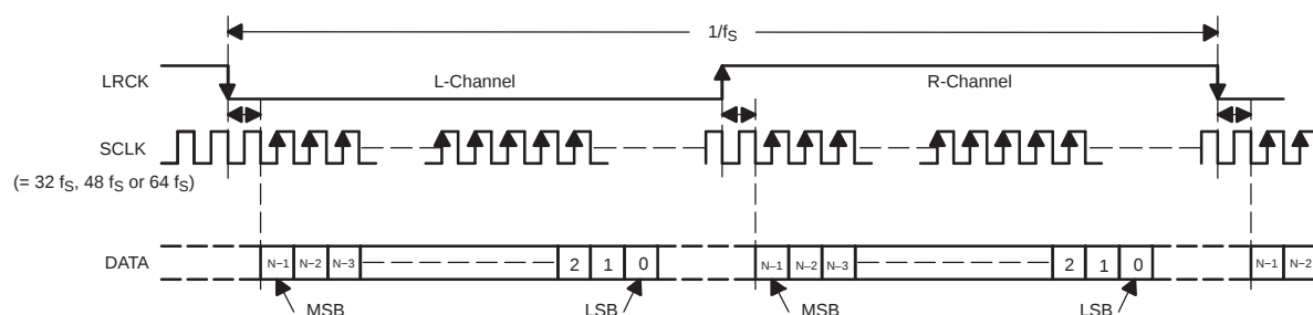
Figure 26. I^2S Format
