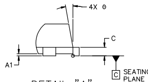
DETAIL "A" SCALED 2:1
