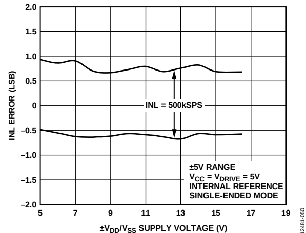
Figure 19. INL Error vs. \pm V_{DD}/V_{SS} Supply Voltage at 500 kSPS
