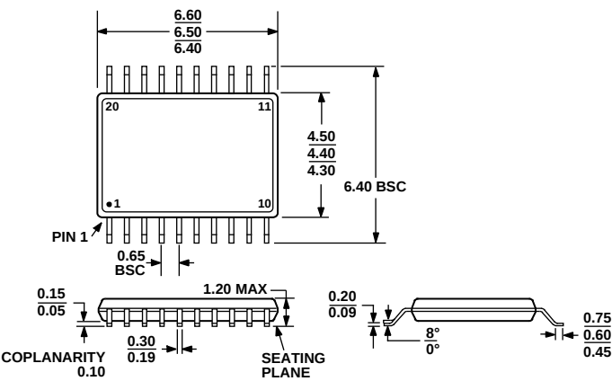
COMPLIANT TO JEDEC STANDARDS MO-153-AC Figure 23. 20-Lead Thin Shrink Small Outline Package [TSSOP] (RU-20) Dimensions show in millimeters
