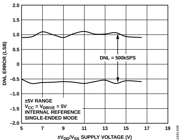
Figure 18. DNL Error vs. \pm V_{DD}/V_{SS} Supply Voltage at 500 kSPS
