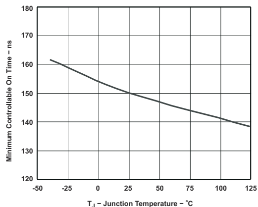
Figure 7-3. MINIMUM CONTROLLABLE ON TIME vs JUNCTION TEMPERATURE
