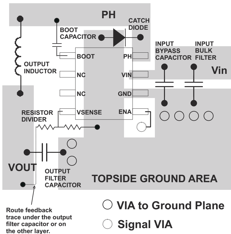
Figure 8-1. Design Layout
