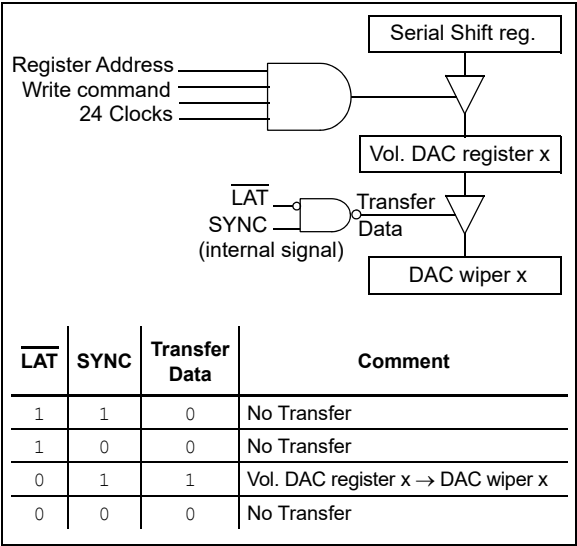
FIGURE 5-8: \overline{\text{LAT}} and DAC Interaction. Since the DAC wiper x is updated from the volatile DAC register x, all DACs that are associated with a given \overline{\text{LAT}} pin can be updated synchronously. If the application does not require synchronization, then this signal should be tied low. Figure 5-9 shows two cases of using the \overline{\text{LAT}} pin to control when the wiper register is updated relative to the value of a sine wave signal.
