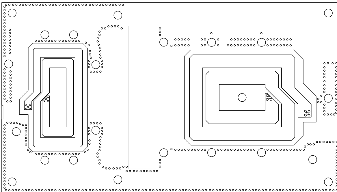
Figure 11. MRF1K80H 87.5–108 MHz Broadband Reference Circuit Component Layout – Bottom
